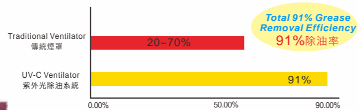
紫外光高效能除油系統效率比較 Efficiency for UV Grease Extraction System
